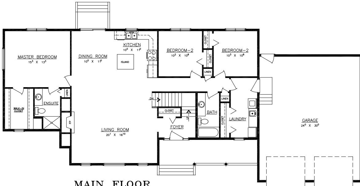
MAIN FLOOR
